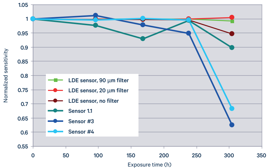
Figure 12 Normalized sensitivity of the sensors during dust test
