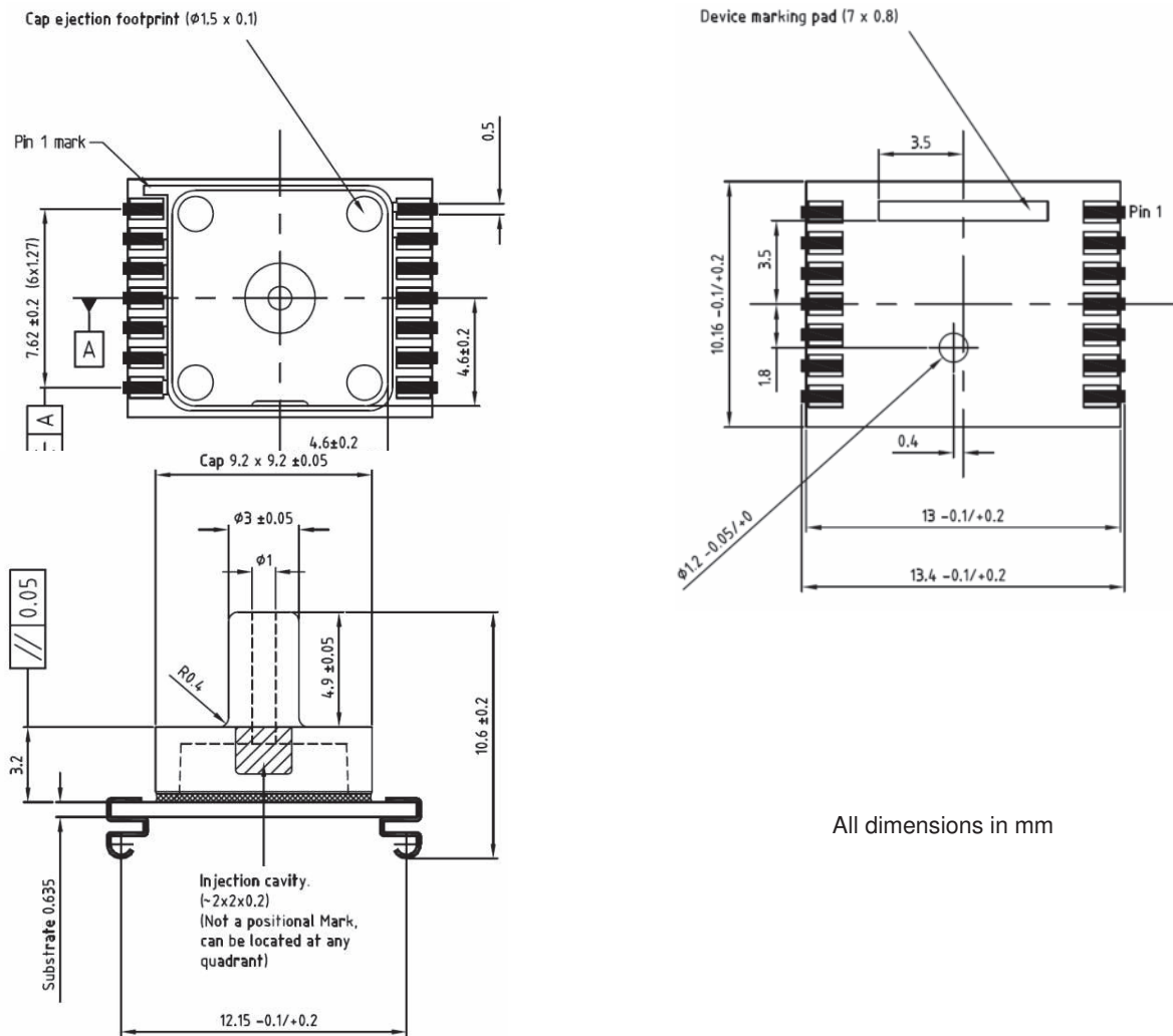
Fig. 8: Device package outlines of MS5536-60C-CPJU
