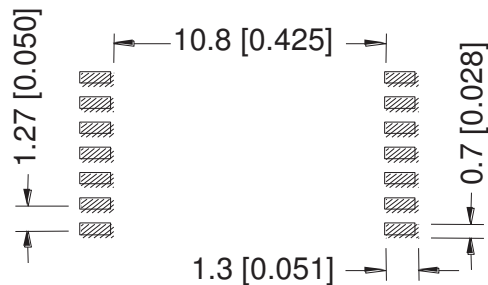
Fig. 9: recommended pad-layout for MS5536-60C-CPJU / MS5536-60C-CNJU
