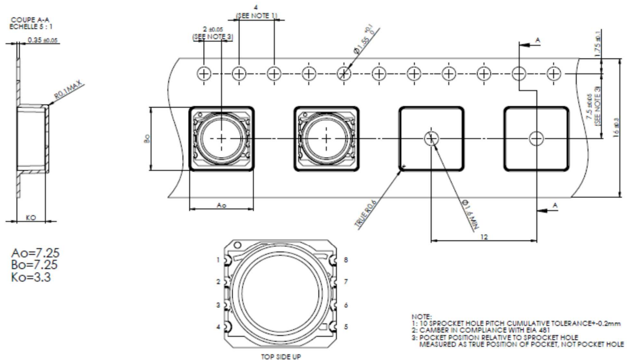
Figure 23: MS5803-07BA Tape &amp; reel shipping package
