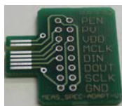
Internal connection
